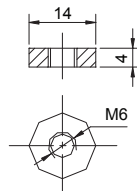
Terminal (M6)
