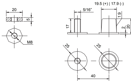
Terminal (M8)
