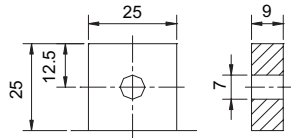
Terminal (F9)
